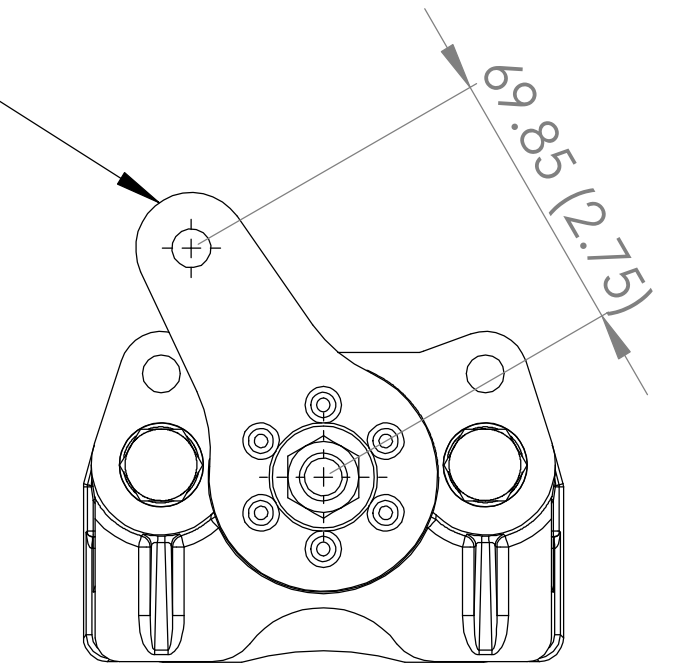
PARK BRAKE DETAIL VIEW SCALE 1:2
